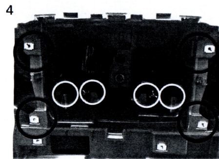
4 Unscrew and remove the head-unit from the dashboard and save the screws.
