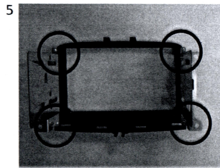
5 Fix the supplied brackets on the supplied fascia plate as shown in the picture.
