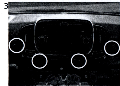
3 Unscrew, remove and save the dashboard air-vents as shown in the picture.
